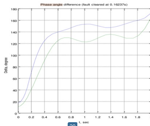
Figure-6. The rotor angle response for base case condition at fault on bus 7 for interruption time for 0.16237 seconds.
