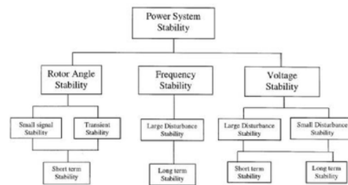
Figure-1. Classification of Power System Stability.
